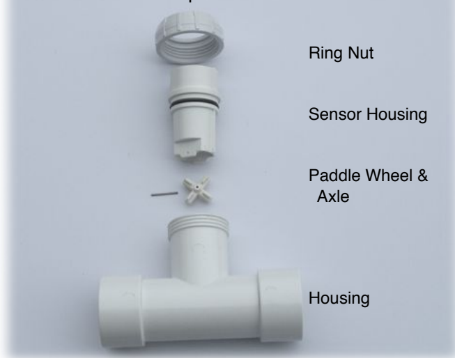
Exploded view.
