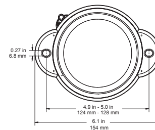
Flange Mount
